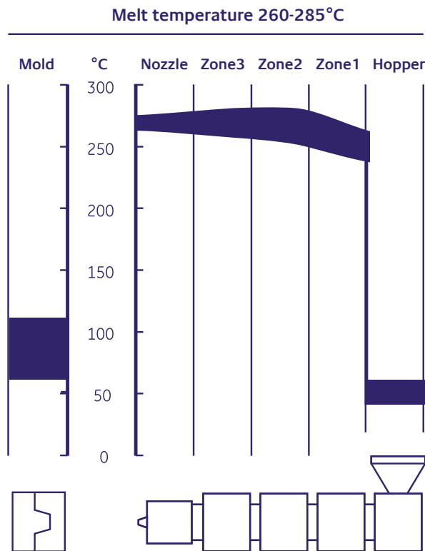
Figure 14 – Typical molding temperatures for filled Xenoy resin
